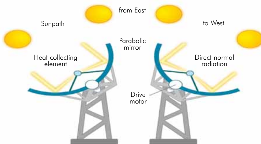
Figure A.2: Illustration of Parabolic Trough Collectors and Sun Tracking
