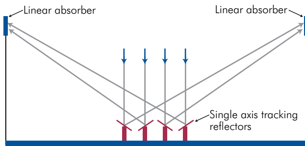
Figure A.6: Example of a CFLR System Source
