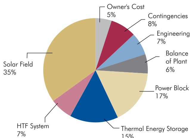
Figure 5.2: CAPEX Breakdown—Parabolic Trough (100 MW – 13.4h TES – US$914m)
