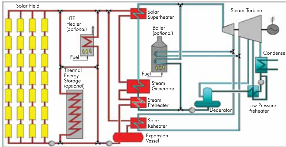
Figure A.3: Basic Scheme of a Parabolic Trough Power Plant
