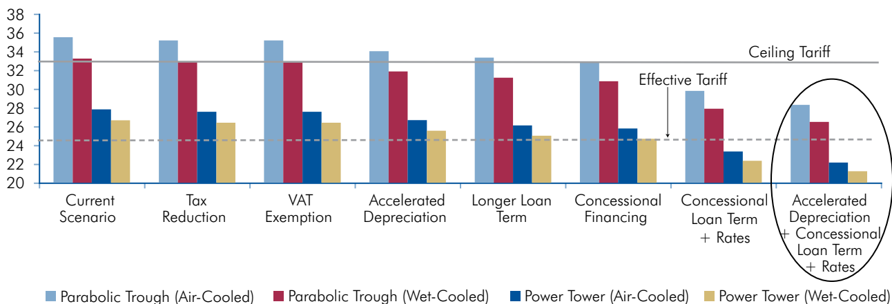
Figure 5.6: Impact Assessment of Different Regulatory Approaches on LCOE in India
