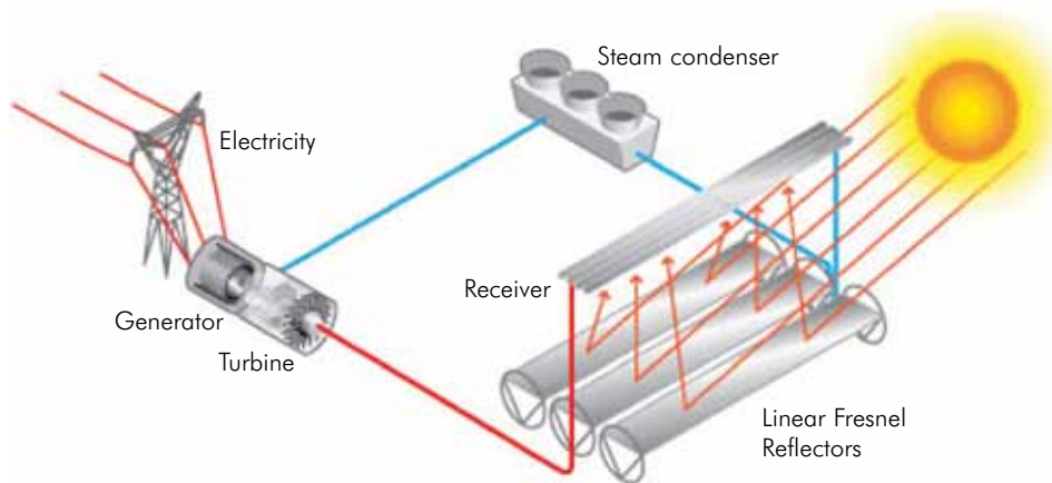
Figure A.4: Linear Fresnel System Diagram
