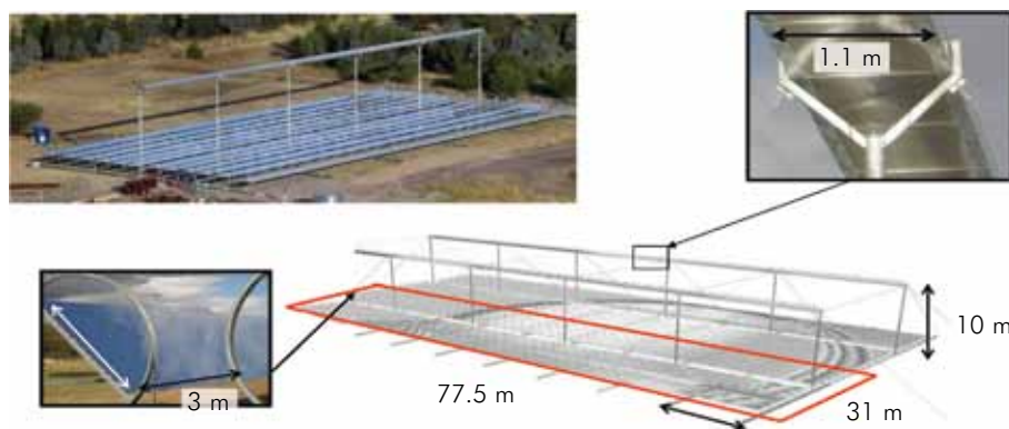
Figure A.5: Views of Linear Fresnel Reflector Arrays
