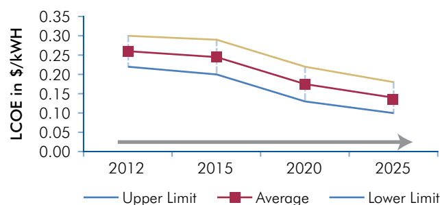
Figure 5.5: LCOE Reduction Potential for CST
