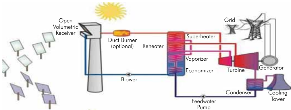
Figure A.7: Schematic of Open Volumetric Receiver Power Tower Plant with Steam Turbine Cycle
