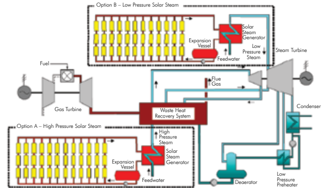
Figure A.13: Basic Scheme of an ISCCS
