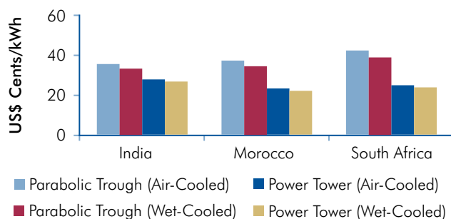
Figure 5.1: LCOEs for Parabolic Trough and Power Tower in India, Morocco, and South Africa
