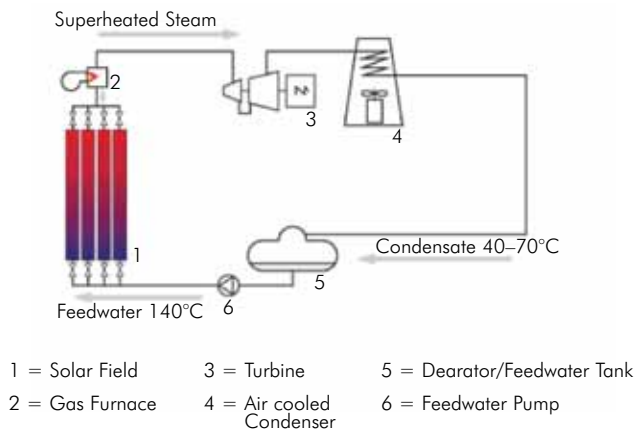
Figure A.12: Saturated Steam Hybrid Plant Configuration
