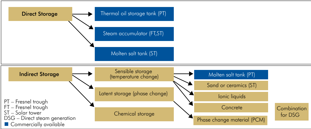
Figure A.11: Storage Concepts for CST
