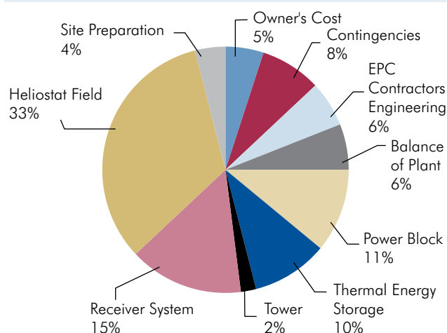
Figure 5.3: CAPEX Breakdown—Power Tower (100 MW – 15 h TES – US$978m)
