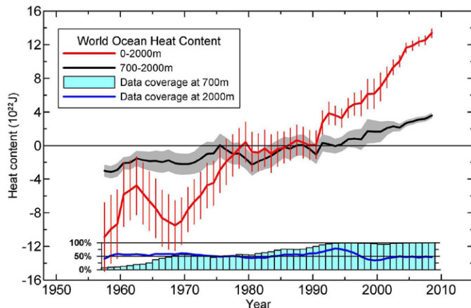
Figure 4: The increase in total ocean heat content from the surface to 2000 m, based on running five-year analyses. Reference period is 1955–2006. The black line shows the increasing heat content at depth (700 to 2000 m), illustrating a significant and rising trend, while most of the heat remains in the top 700 m of the ocean. Vertical bars and shaded area represent \pm 2 standard deviations about the five-year estimate for respective depths.
