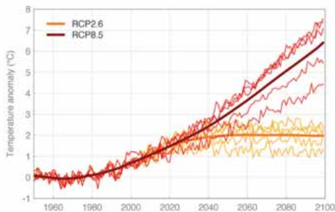
Figure 2.5: Temperature projections for global land area
