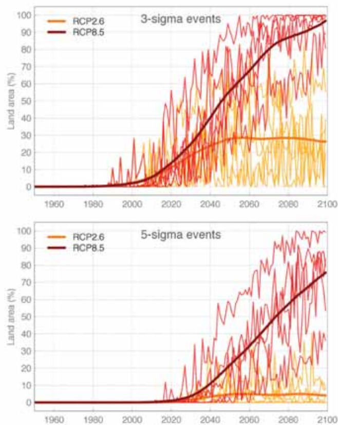
Multi-model mean (thick line) and individual models (thin lines) under RCP2.6 (2°C world) and RCP8.5 (4°C world) for the months of DJF. The multi-model mean has been smoothed to give the climatological trend.
