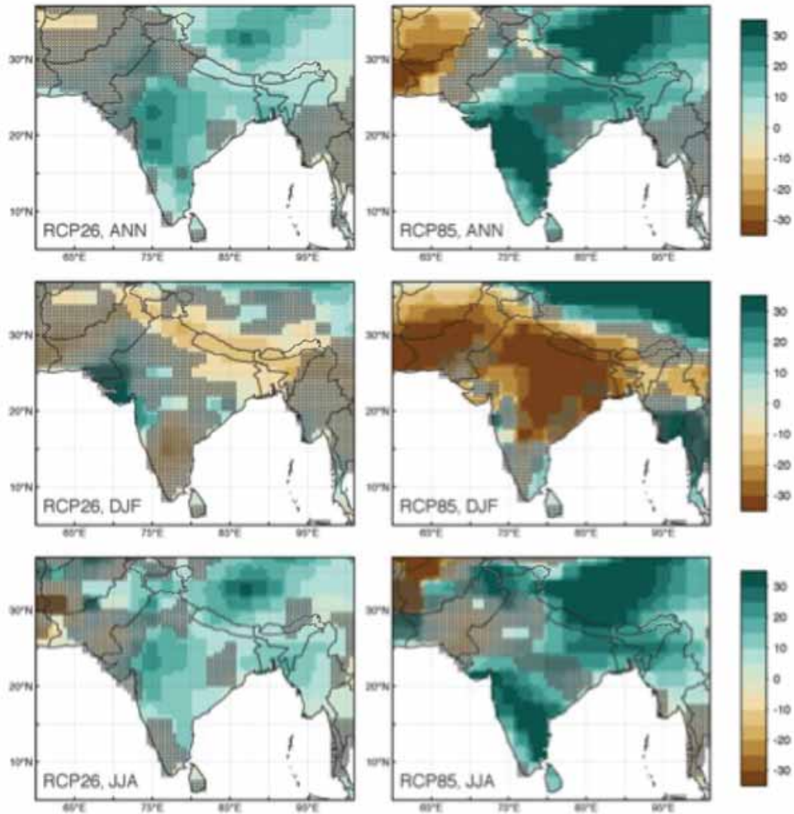
Figure 5.6: Multi-model mean of the percentage change in annual (top), dry-season (DJF, middle) and wet-season (JJA, bottom) precipitation for RCP2.6 (left) and RCP8.5 (right) for South Asia by 2071–99 relative to 1951–80
