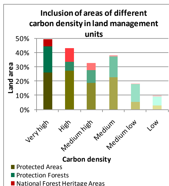
Figure 5: Management designation of areas of different carbon density
