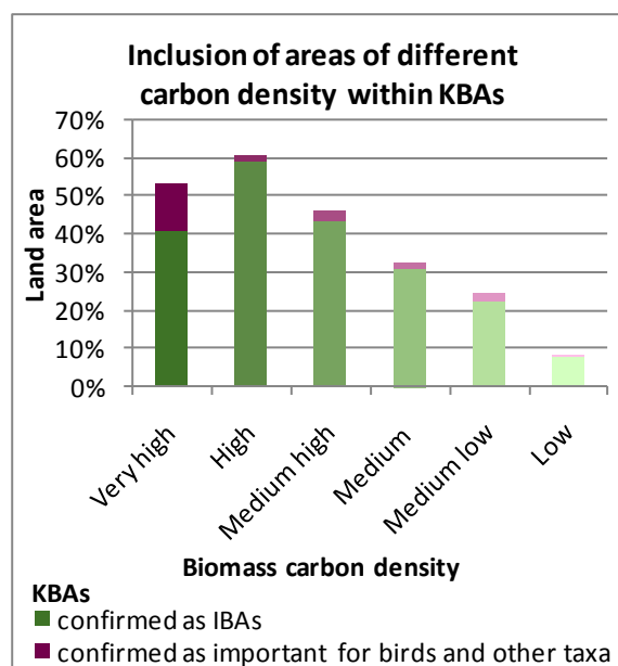
Figure 3: Percentage of Ecuador's land of different carbon density occurring in KBAs
