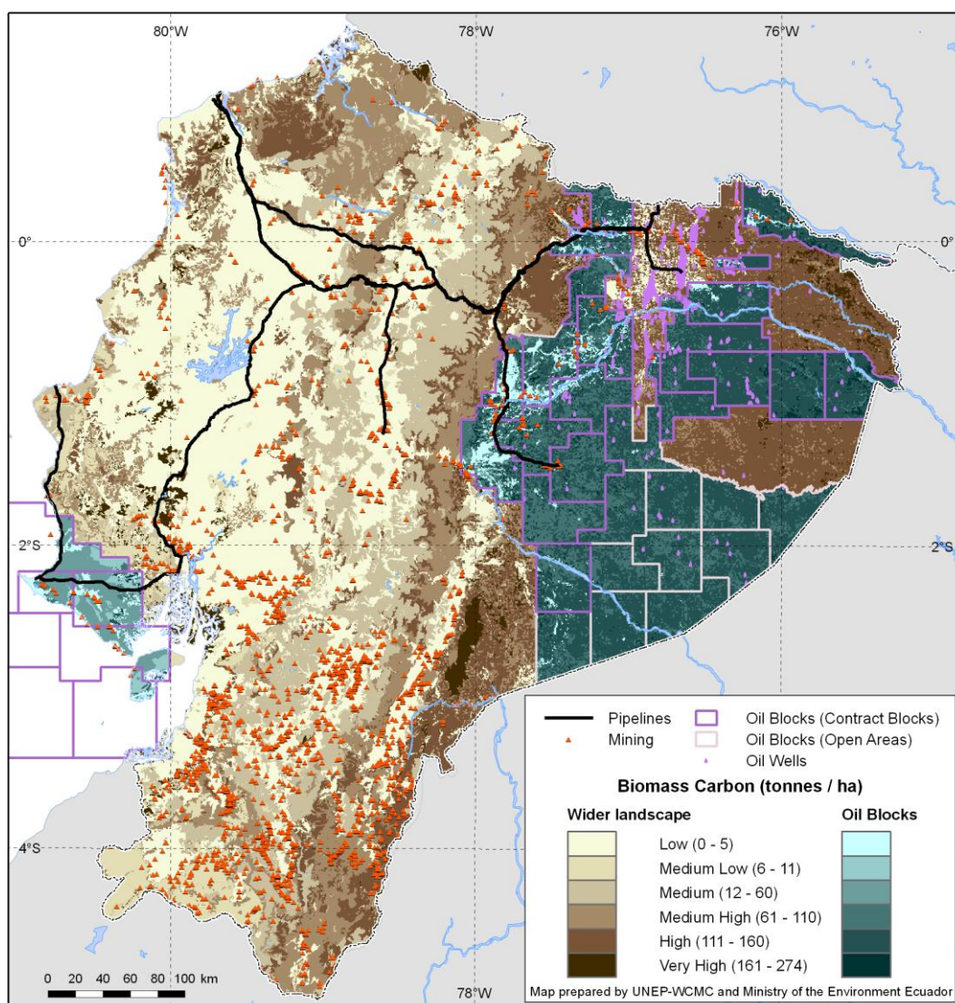
Map 11: Oil, gas and mining activities in relation to biomass carbon
