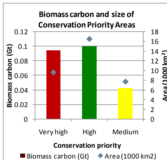
Figure 4: Biomass carbon in areas of very high, high and medium conservation priority
