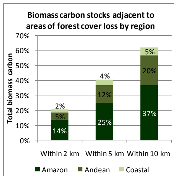
Figure 9: Biomass carbon stocks around areas of forest cover loss by region
