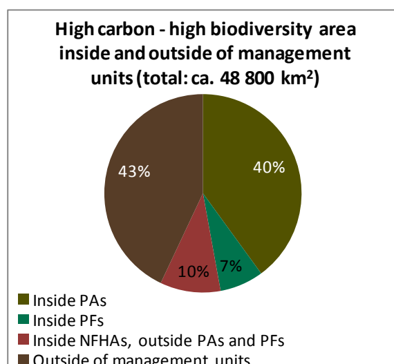
Figure 6: Distribution of high carbon - high biodiversity area among different land management types
