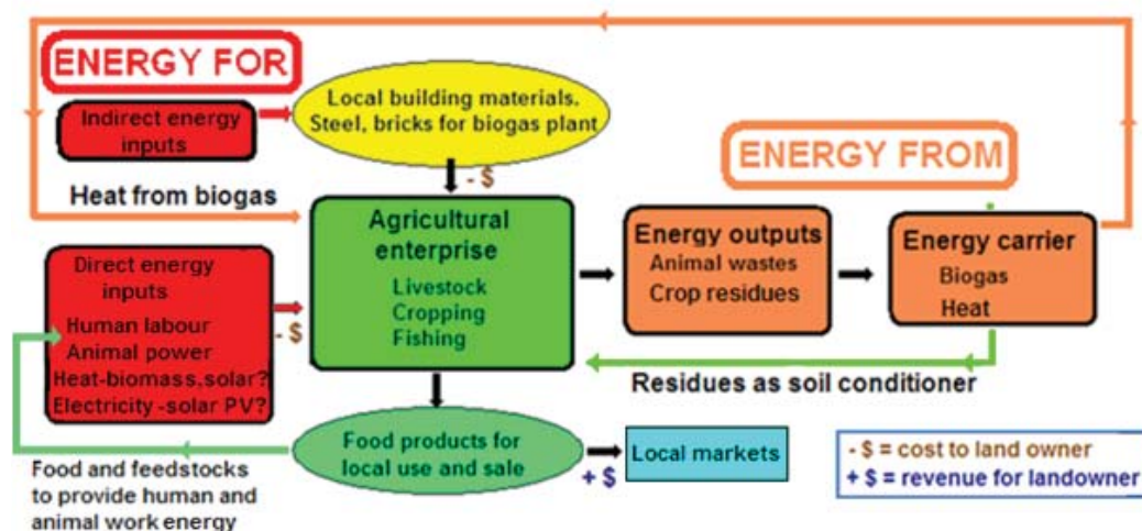
Figure 2. Example of a ‘small-scale’, low-input, family-managed, farming enterprise showing energy flows through the system. Outputs are primarily fresh food for local consumption, although they may also be delivered to local processing companies. Along with human and animal power, some direct energy inputs can be obtained from other sources, such as solar thermal and solar PV systems and biogas produced using a simple anaerobic digester.
